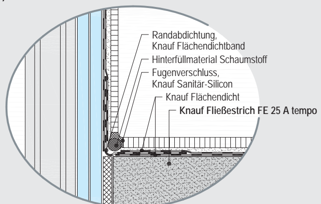
Heizestrich (Bauart B)
